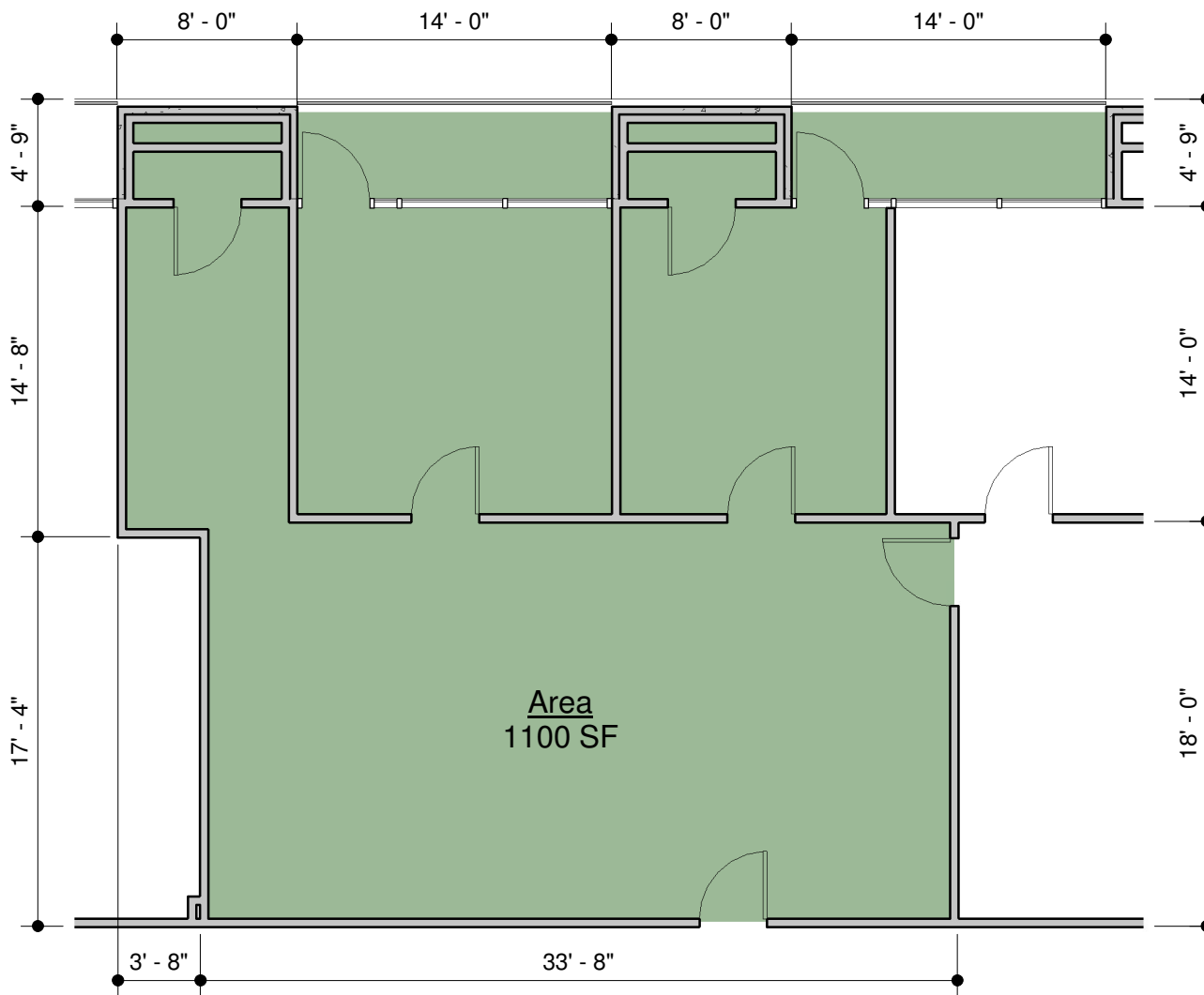
FLOOR PLAN
