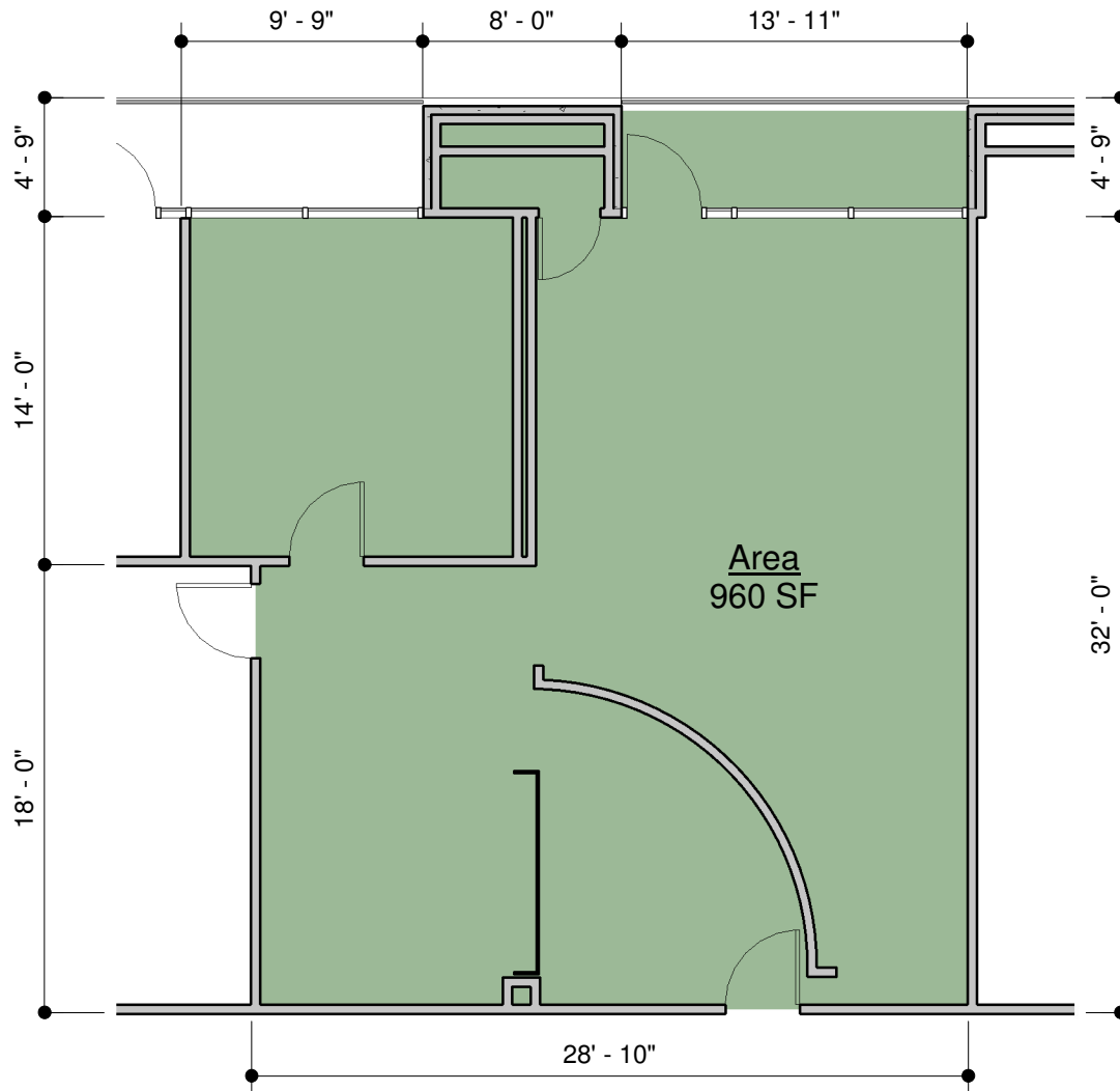
FLOOR PLAN
